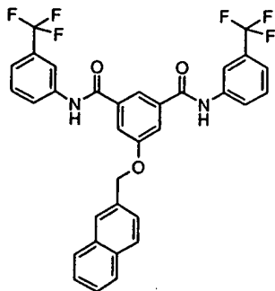
Compound # 42
